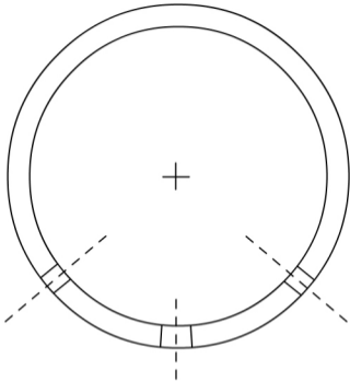
PVC Pipe 3/8 " Holes - 3 Rows Every 6" For Length of Pipe
